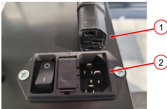
Figure 31 Connection Speed Controller VARGA VA 11
